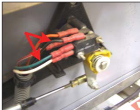
Figure 13 - Neutral Lockout Cam
