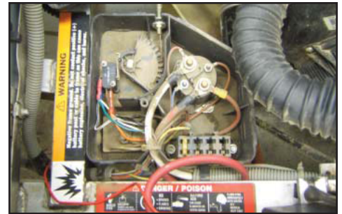
Figure 7 - Remove Solenoid Compartment Cover
