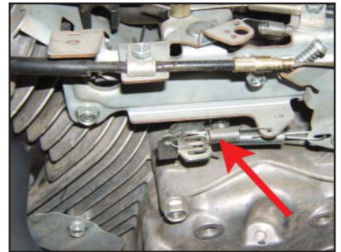
Figure 14 - Factory Idle Spring
